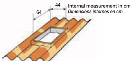
Sheet for skylight / Plaque châssis
